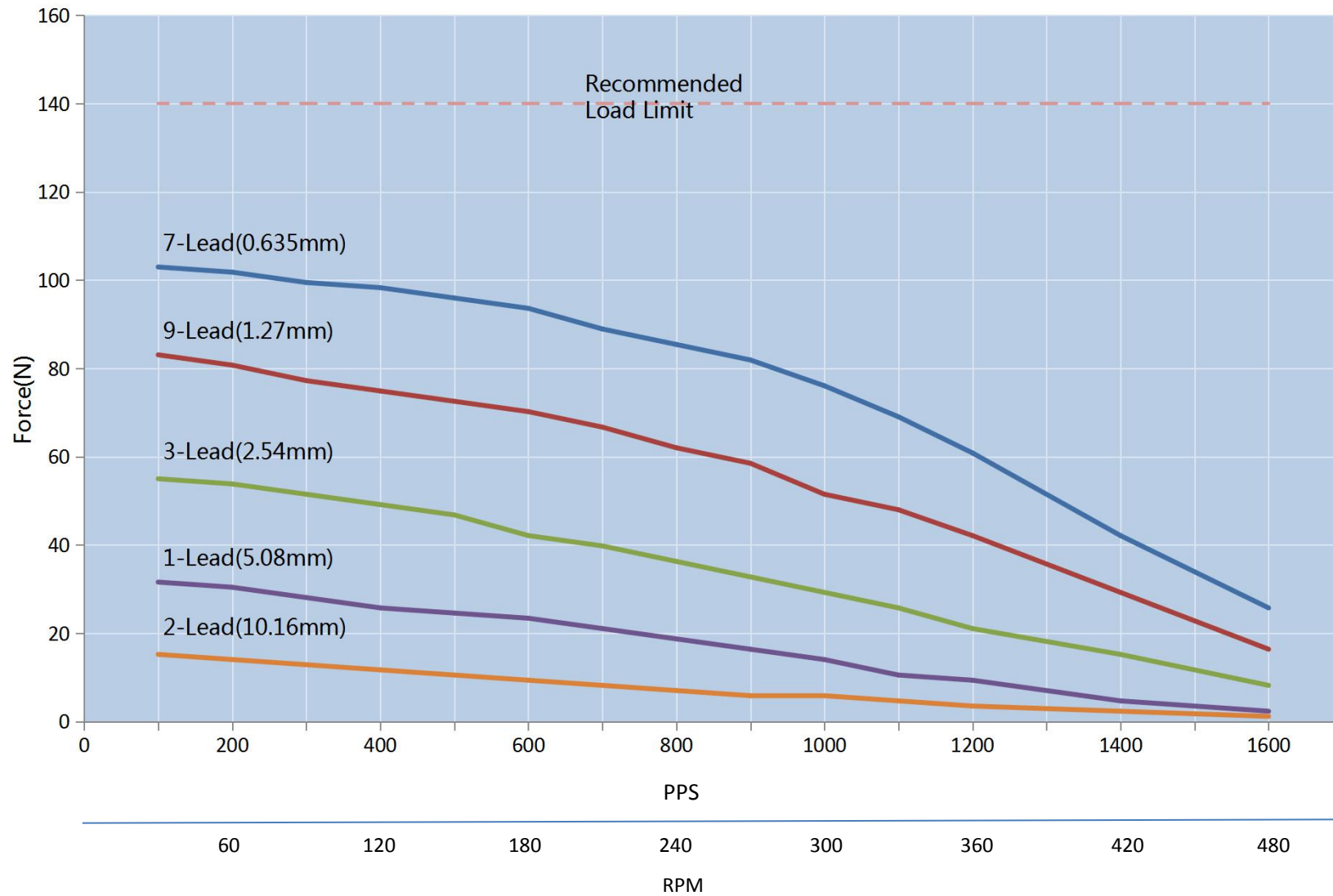
Nema 11 linear steppers double stack(24V)
