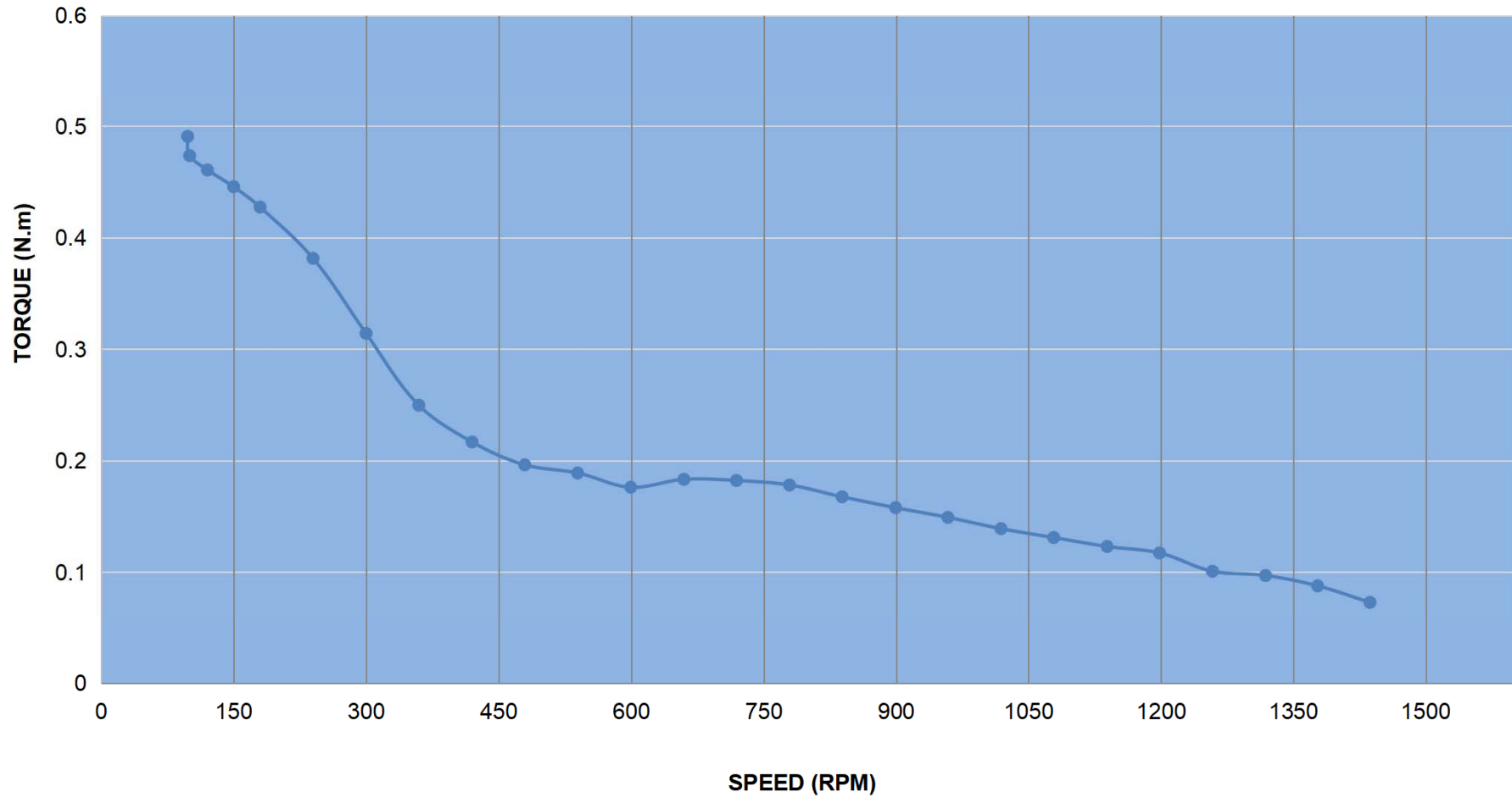
PULL OUT TORQUE CURVE OF 17BK05-05
