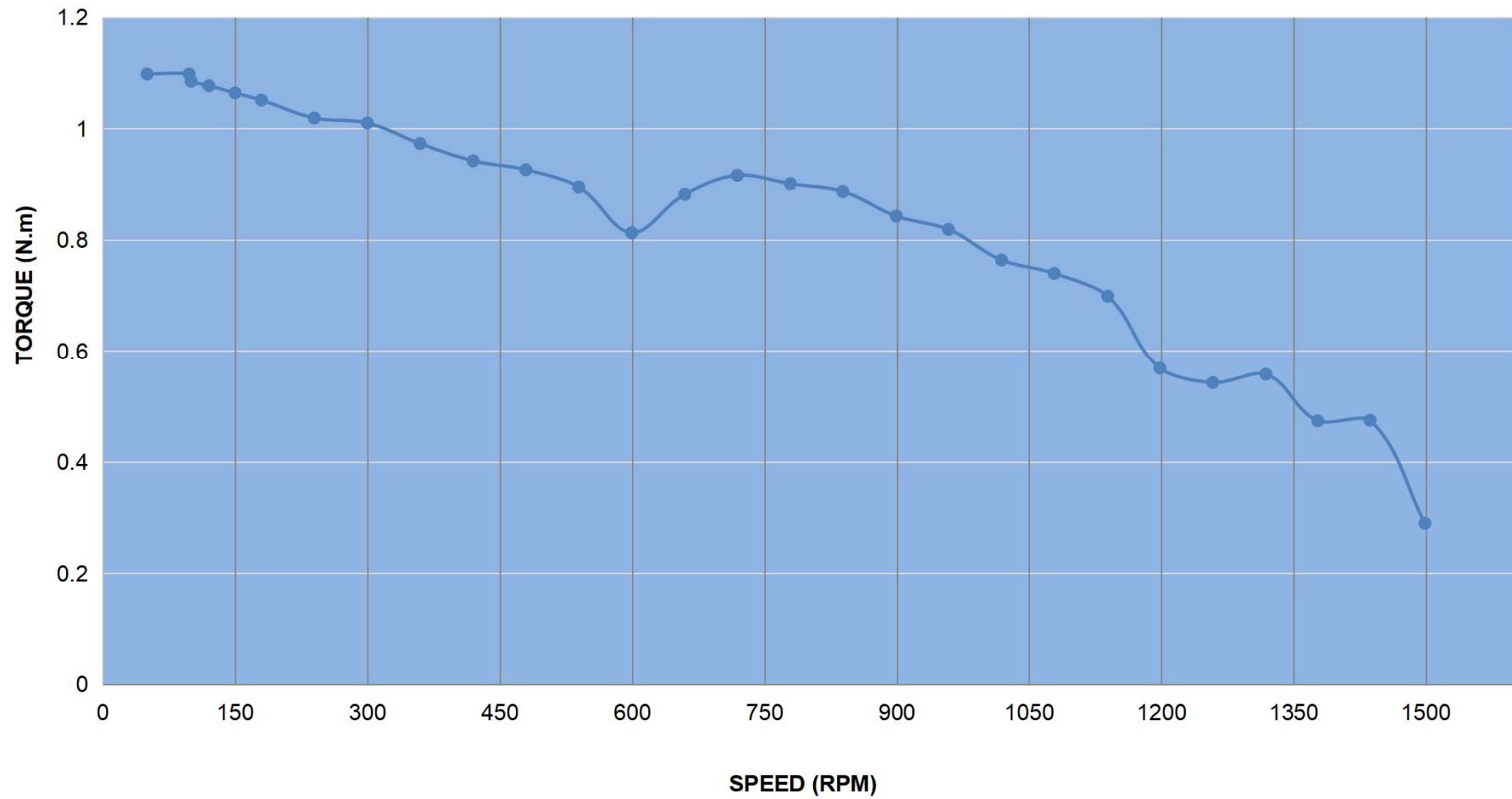
PULL OUT TORQUE CURVE OF 23BK20-12
