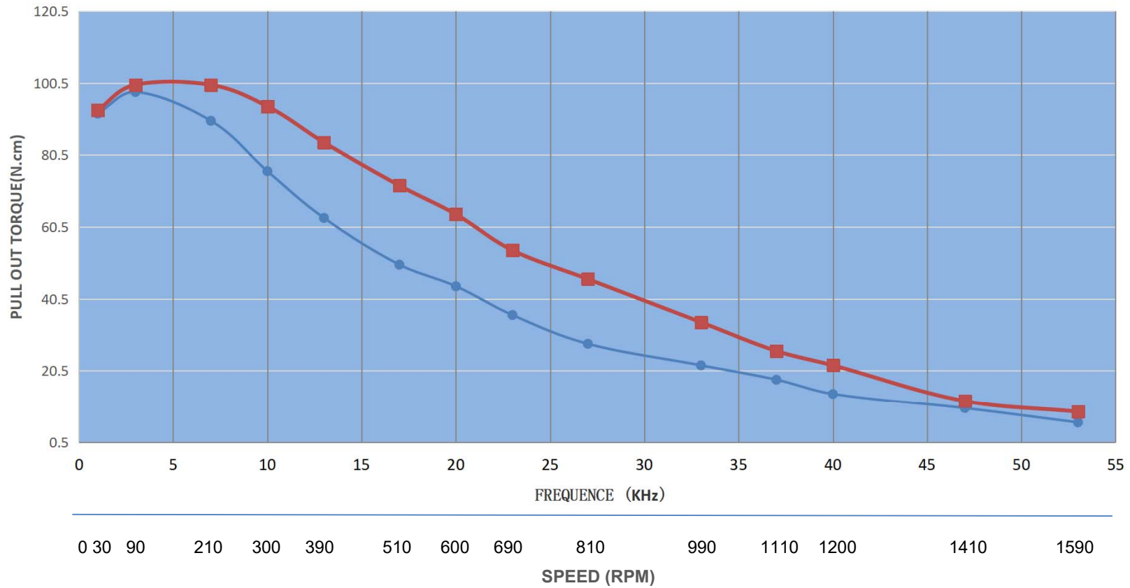
PULL OUT TORQUE CURVE OF 23HS20-2004S
