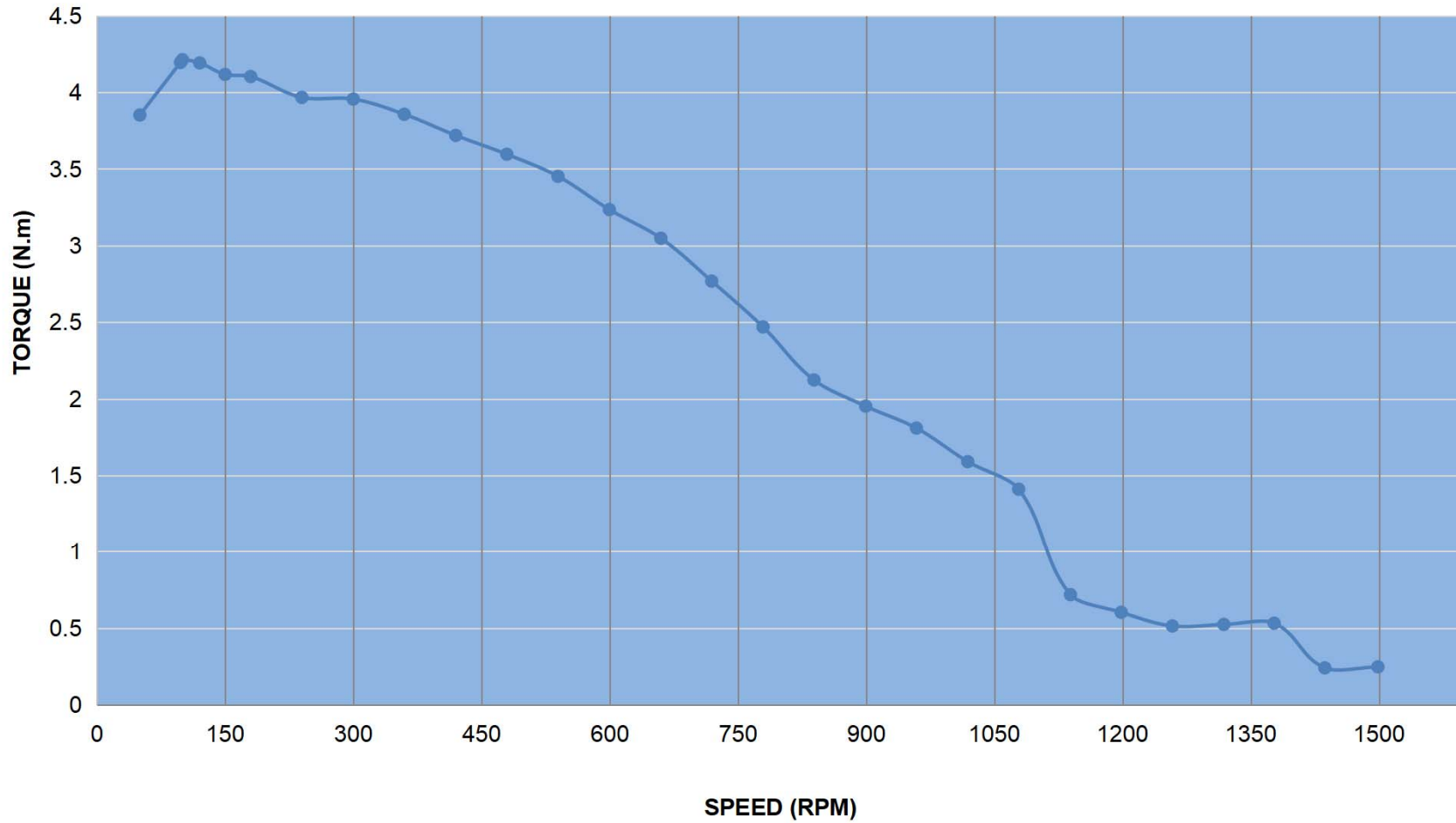
PULL OUT TORQUE CURVE OF 34E1K-45
